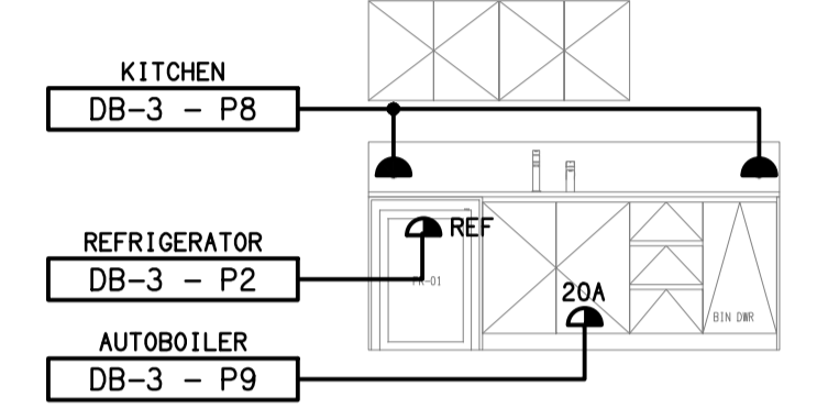
DETAIL C SERVICE KITCHENETTE SCALE 1:50
